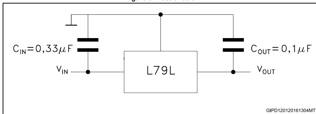
Figure 3: Test circuit
